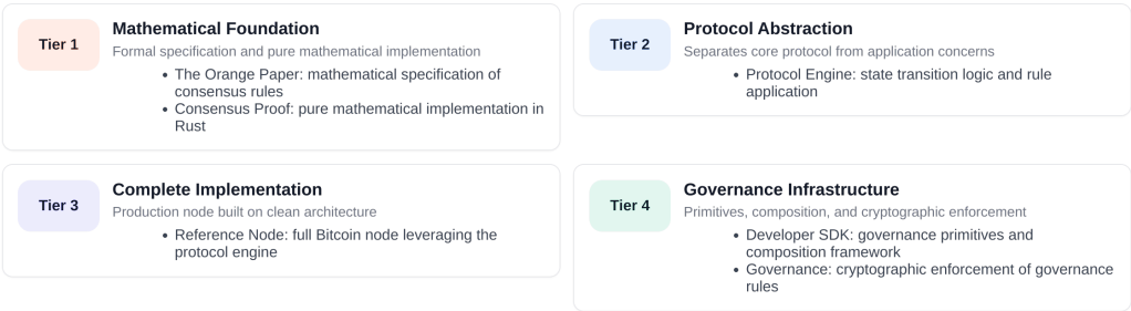
Figure: Tiered architecture: Tier 1 = Orange Paper + Consensus Proof (mathematical foundation); Tier 2 = Protocol Engine (protocol abstraction); Tier 3 = Reference Node (complete implementation); Tier 4 = Developer SDK + Governance (governance infrastructure).
