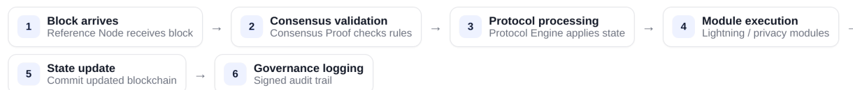
Figure: End-to-end data flow through Reference Node, Consensus Proof, Protocol Engine, modules, and governance. Each tier depends only on layers below; modules cannot affect consensus.
