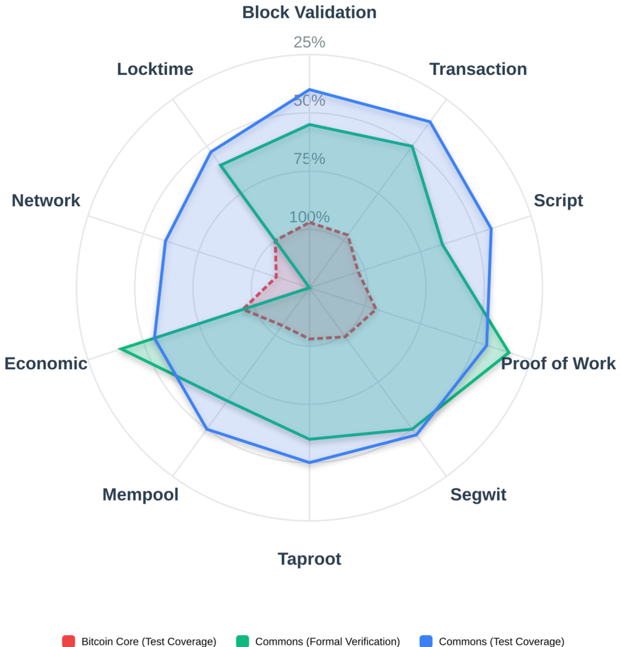
Figure: Consensus coverage comparison: Bitcoin Core achieves 25% coverage through testing alone. Bitcoin Commons achieves 65% formal verification coverage (172 Kani proofs) plus 77% test coverage. Commons uses 93 consensus-focused test files with 667+ test functions compared to Core's 316 total files (only ~53 consensus-focused). The mathematical specification enables both formal verification and comprehensive testing.
