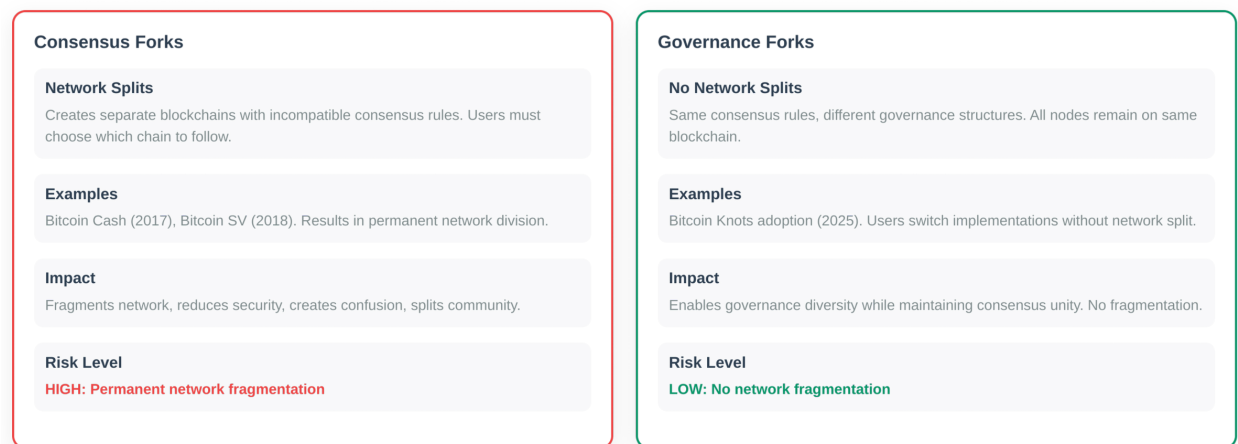
Figure: Fragmentation analysis showing that governance forks don't split the network. All implementations validate same Bitcoin consensus while enabling governance competition.
